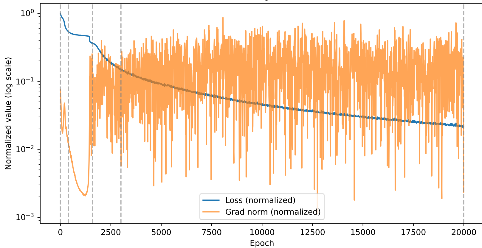
Seed 0 Training (stride=10)
